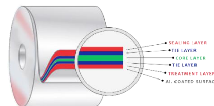
METALLIZED FILM
