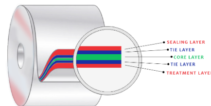
TRANSPARENT FILM
